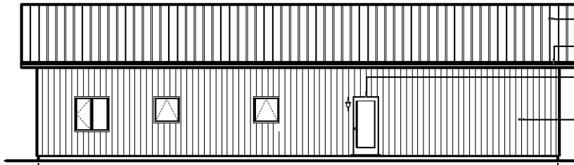
BACK ELEVATION
